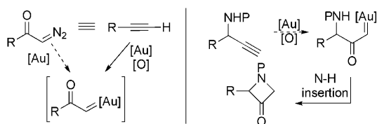
Scheme 1. Formation of azetidin-3-ones through alkyne oxidation.
